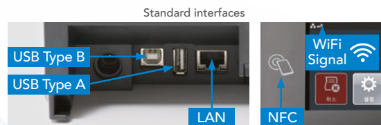
Interface options
