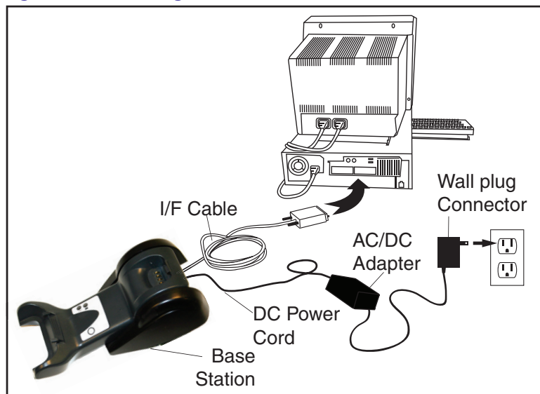
Figure 4. Connecting the Base Station
