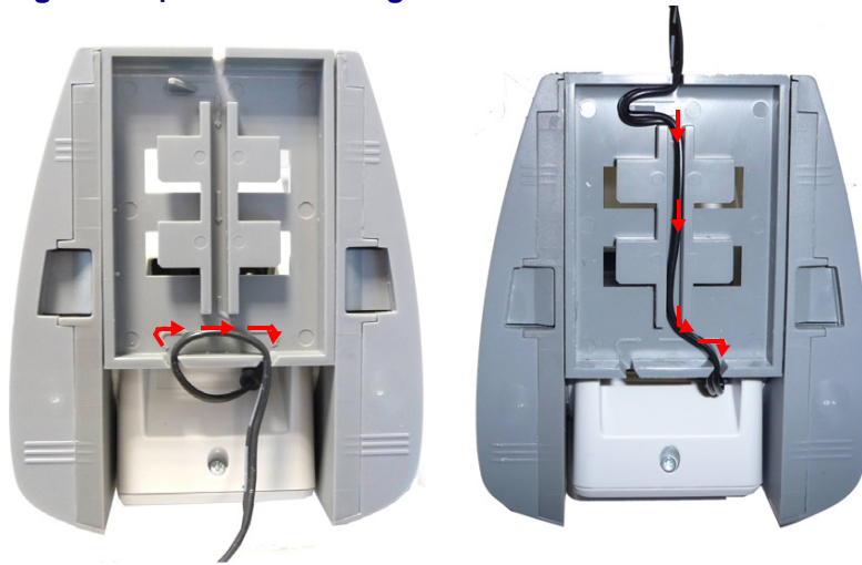
Figure 5. Options for routing the DC cord
